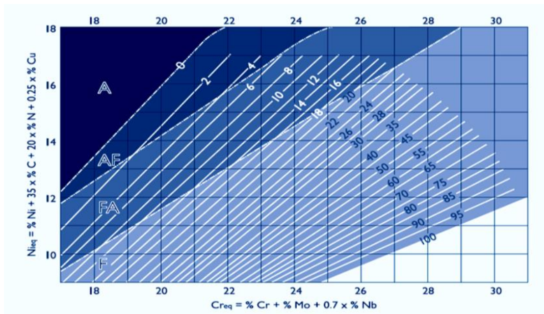
Figure 2. The Schematic diagram of the WRC
