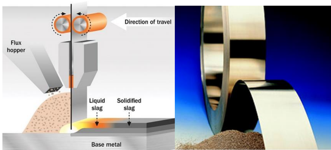
Figure 1. An electro slag coating machine with a strip electrode and coated pressure vessel surface
