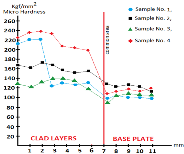
Figure 11. Hardness diagram of cladding layers
