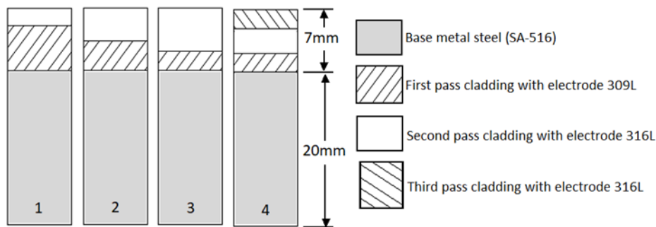
Figure 3. The thickness of the coated layers of different samples
