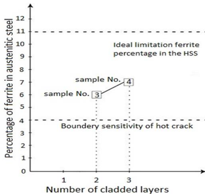
Figure 10. Effect of three coating layers on the percentage of ferrite.
