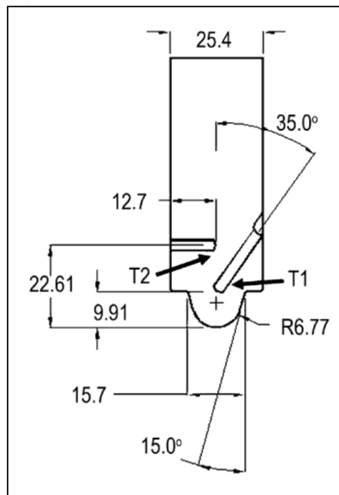
Figure3. FSW tool and K-thermocouples [29]
