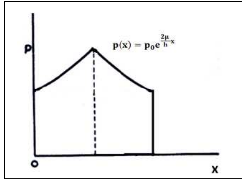
Figure1. Rolling force distribution
