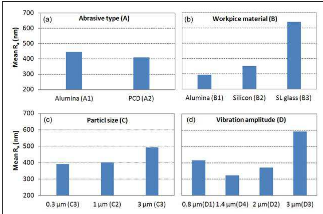
Figure3. Effect of process parameters on R_a (raw data)
