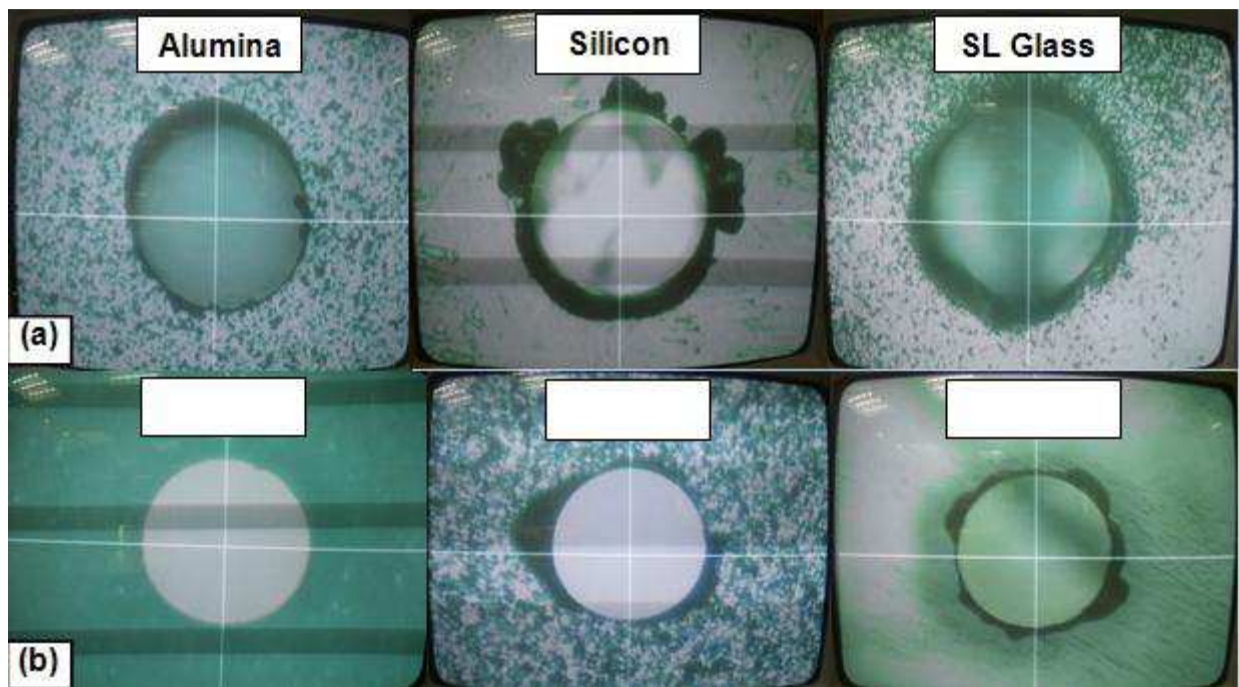
Figure6. Edge chipping in the machined micro hole: (a) entrance, (b) exit
