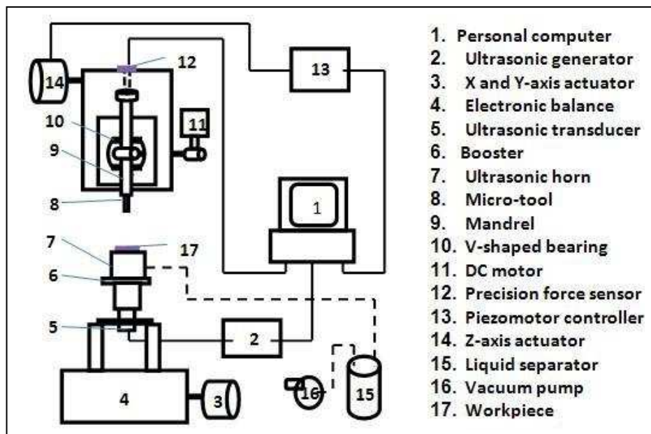
Figure2. Schematic diagram of in-house developed micro-USM system
