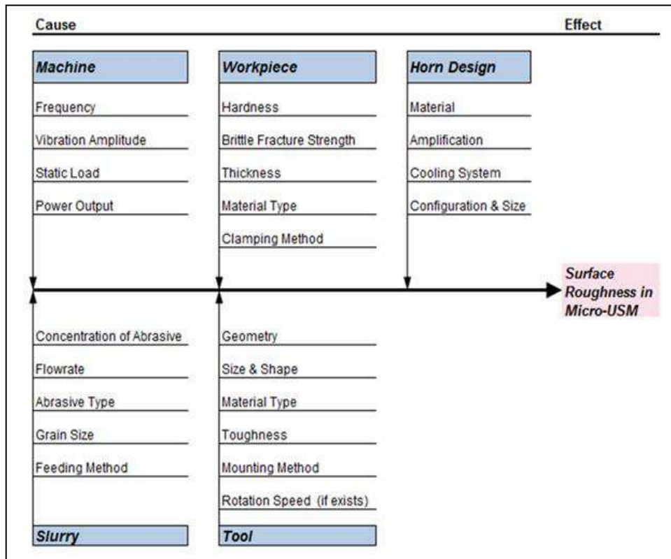
Figure1. Cause-and-effect diagram for surface roughness in micro-USM
