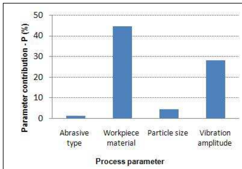
Figure5. Percentage contribution of various parameters to surface roughness
