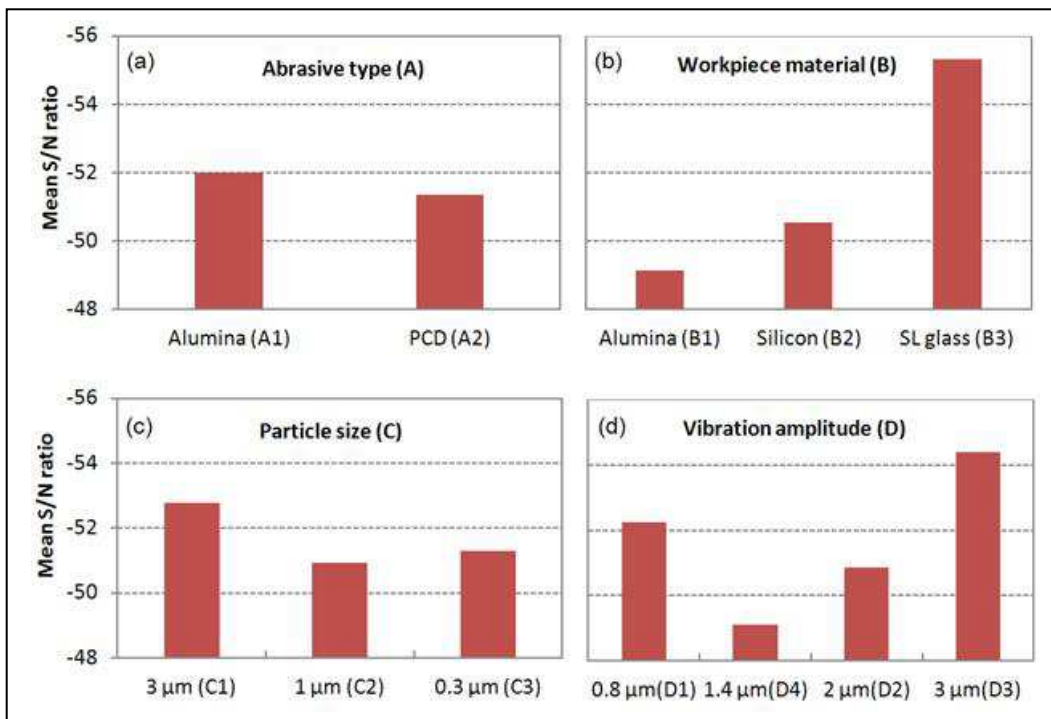
Figure4. Effect of process parameters on R_a (S/N ratio)
