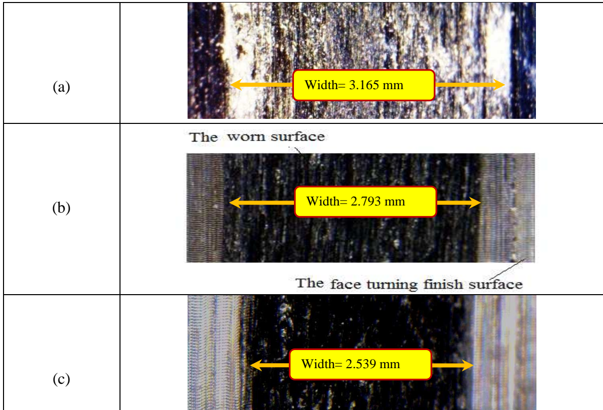
Figure 6. Morphologies of wear scars of three kinds of un-textured surface and textured surfaces according to the condition of V_c = 35 m/min, f = 0.205 mm/rev and UAT d1 , after the distance of 300 m at the velocity of 0.2 m/s; (a) CT, (b) UAT a1 , (c) UAT a2 .
