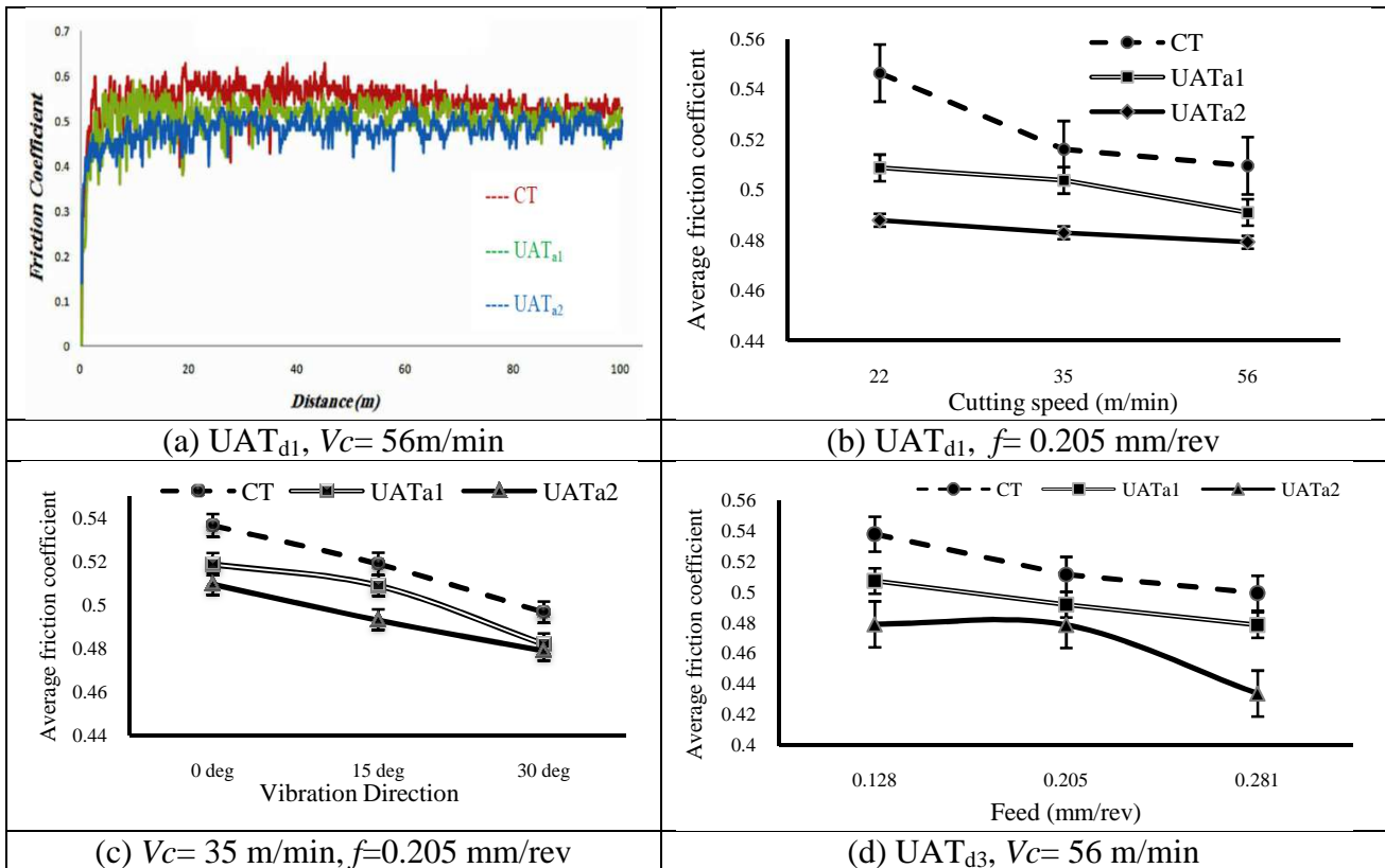
Figure 5. a) Measurement of the friction coefficient, comparison of friction coefficient in CT, UAT a1 and UAT a2 with the different values of (b) cutting speed, (c) vibration direction, (d) feed.
