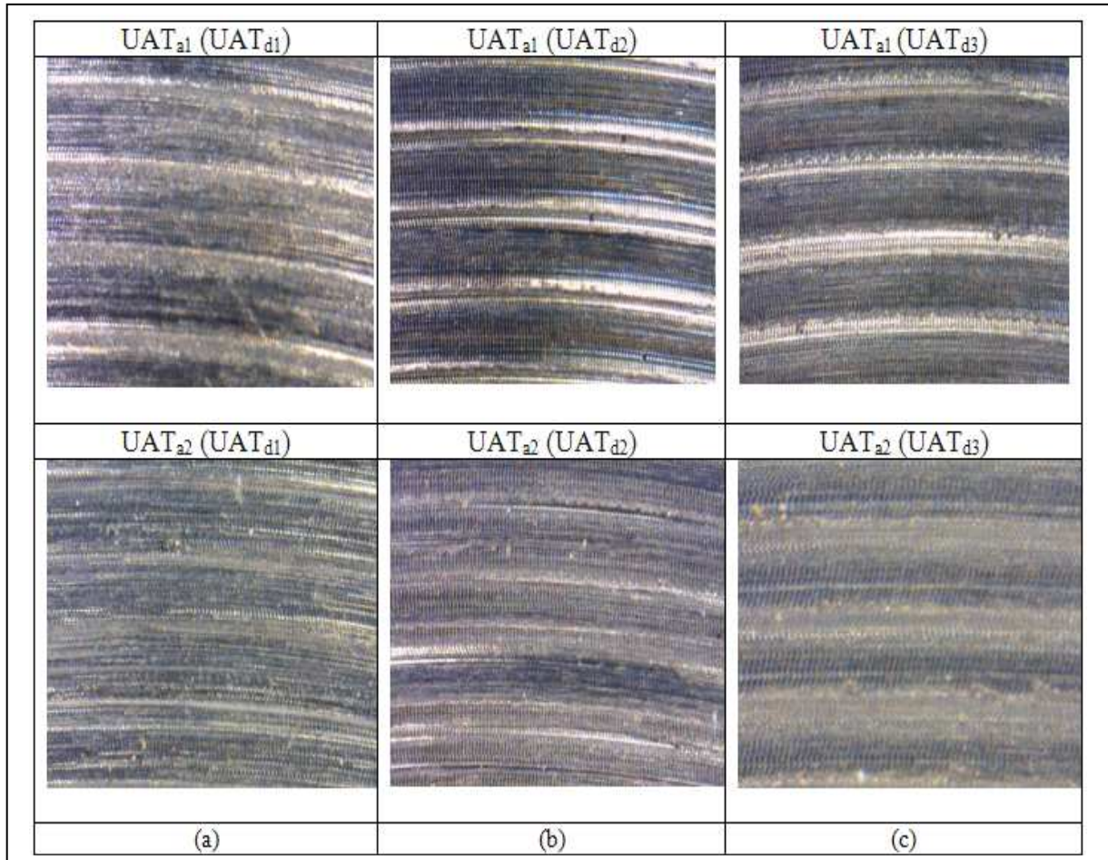
Figure4. Comparison of surface texture for the V_c of 56 m/min and feed of 0.281 mm/rev according to the different vibration directions; (a) 0^\circ , (b) 15^\circ , (c) 30^\circ .
