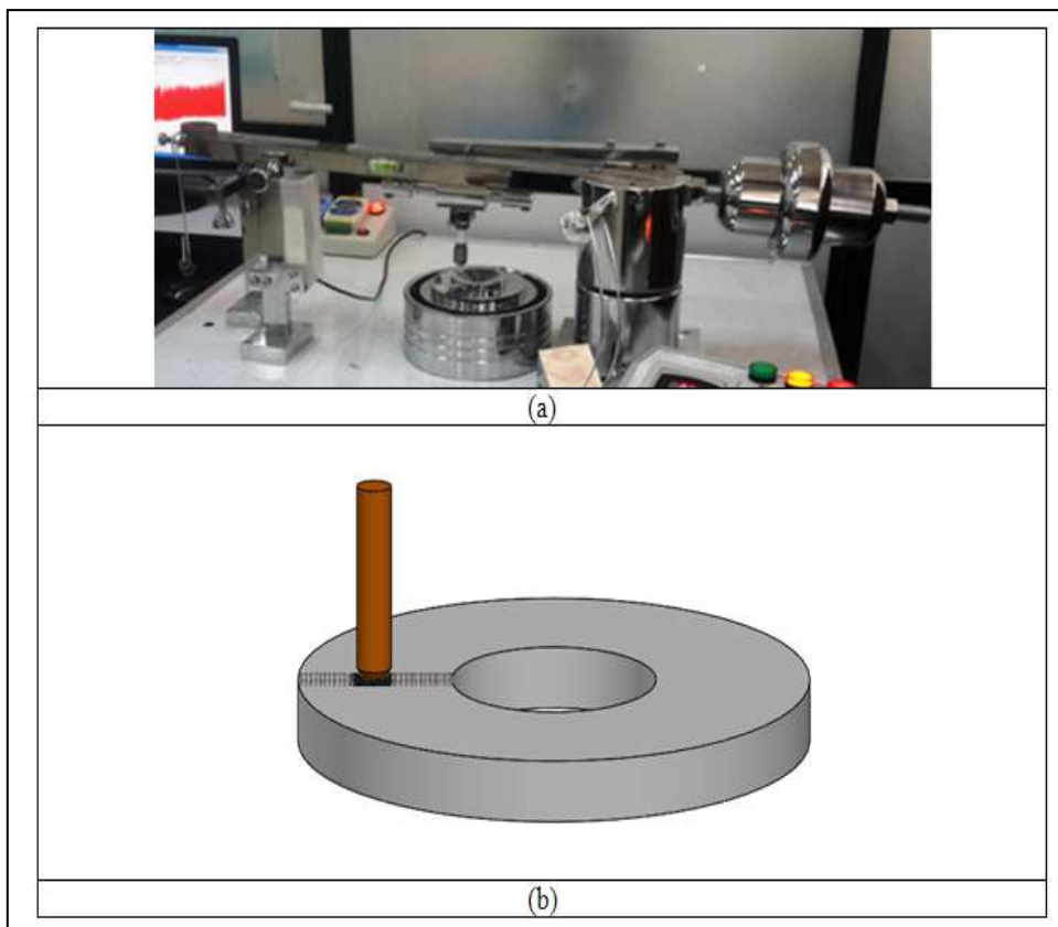
Figure2. Setup for friction and wear evaluation tests; (a) pin on the disk test machine, (b) schematic view of the surface sliding against the chrome steel pin.
