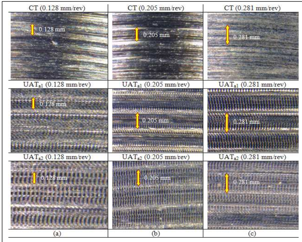
Figure3. Comparison of surface texture for the vibration angle of 15^\circ according to the influence of V_c of 56 m/min and different feed levels.
