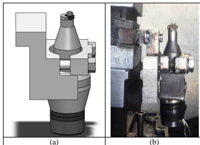
Figure 1. a) 3D model of the designed vibro-tool sets, installation modes of the fixture.
