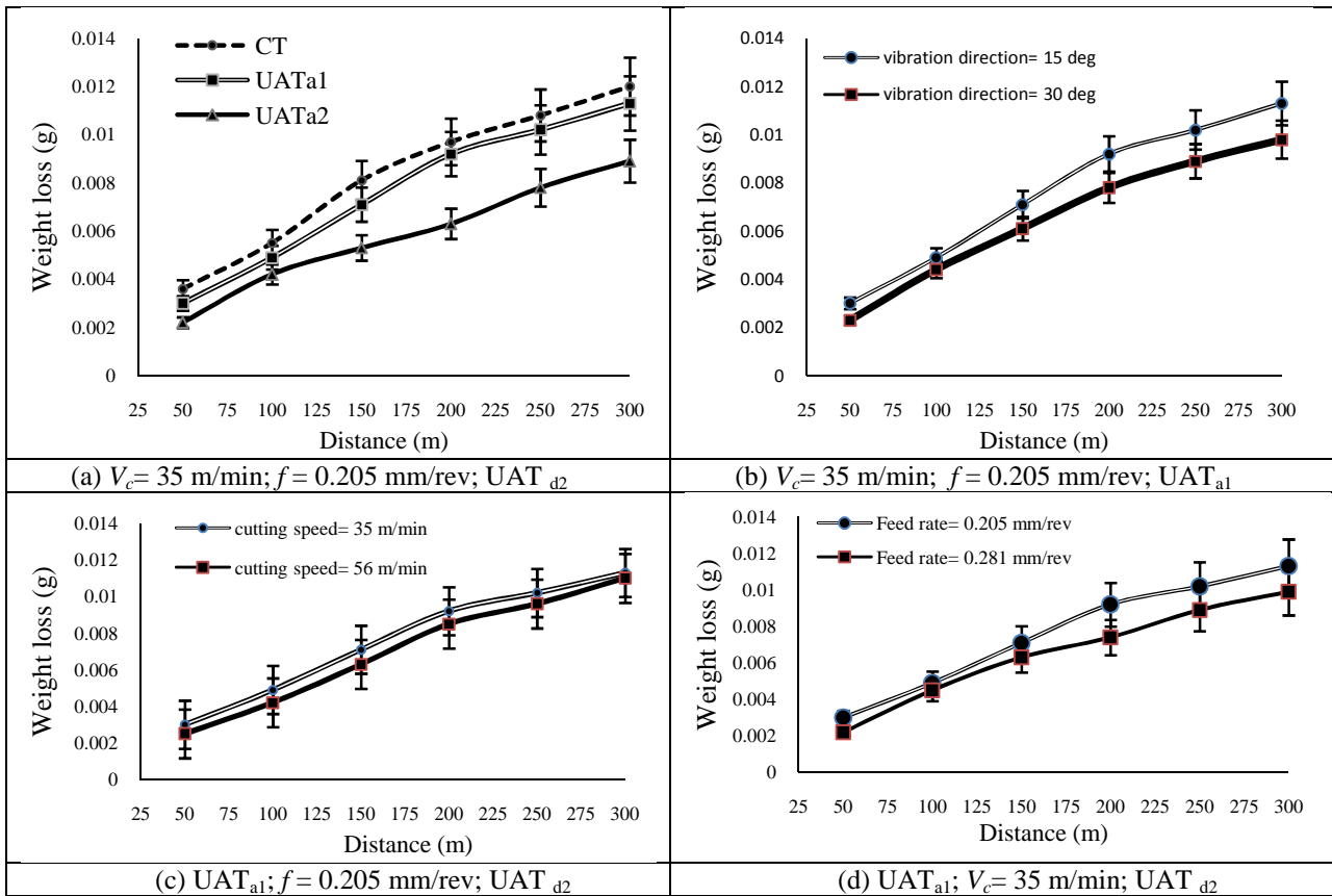
Figure 7. Weight loss of the worn sample's surfaces ;(a) vibration amplitude, (b) vibration direction, (c) cutting speed, (d) feed.
