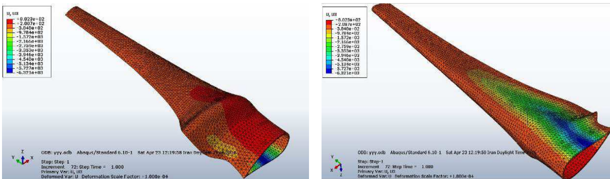
Figure 8. Vertical displacement contours
