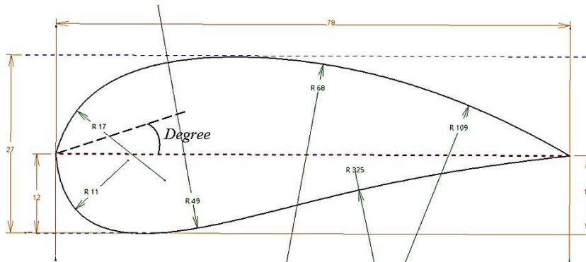
Figure 6. Angle and length in first chord degree
