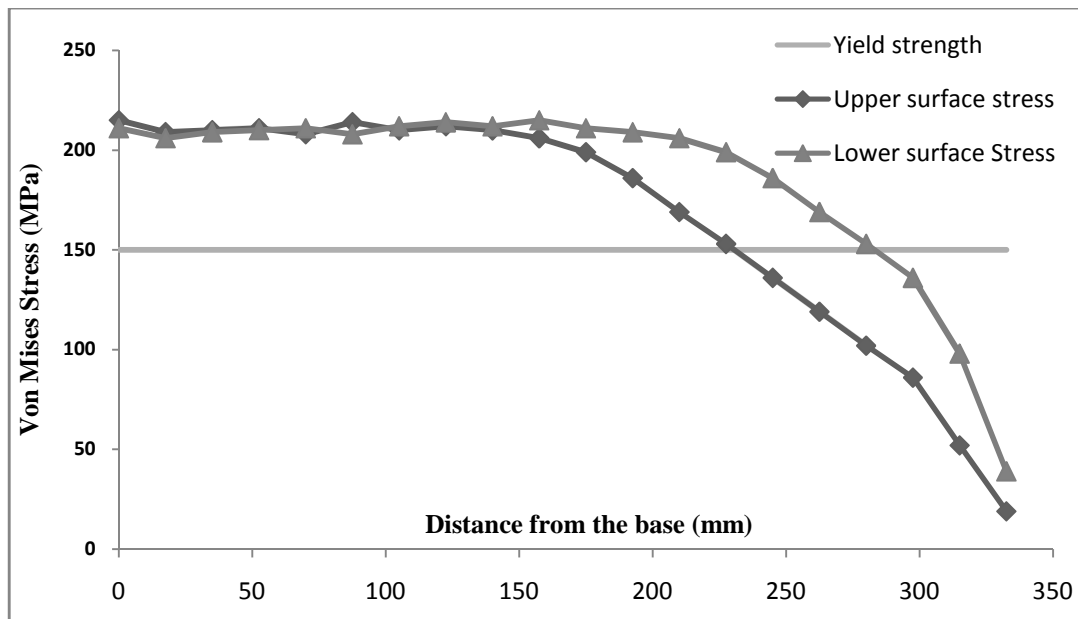
Figure. 14. Von Mises stress distribution on length
