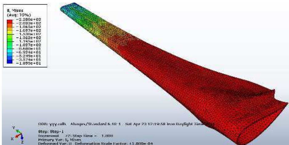
Figure 13. Von Mises stress contour
