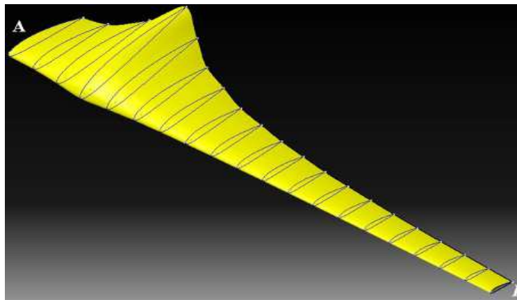
Figure 5. Selected section on the blade (20 sections)
