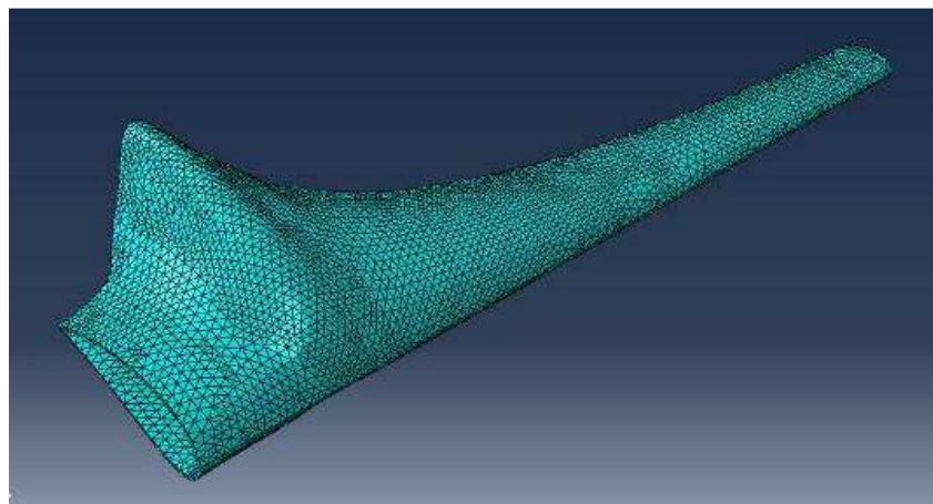
Figure7. A sample finite element mesh generated for blade
