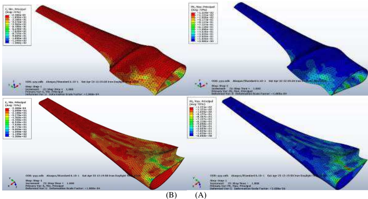
Figure 9. (A) Minimum strain and (B) maximum of two facades curving blade
