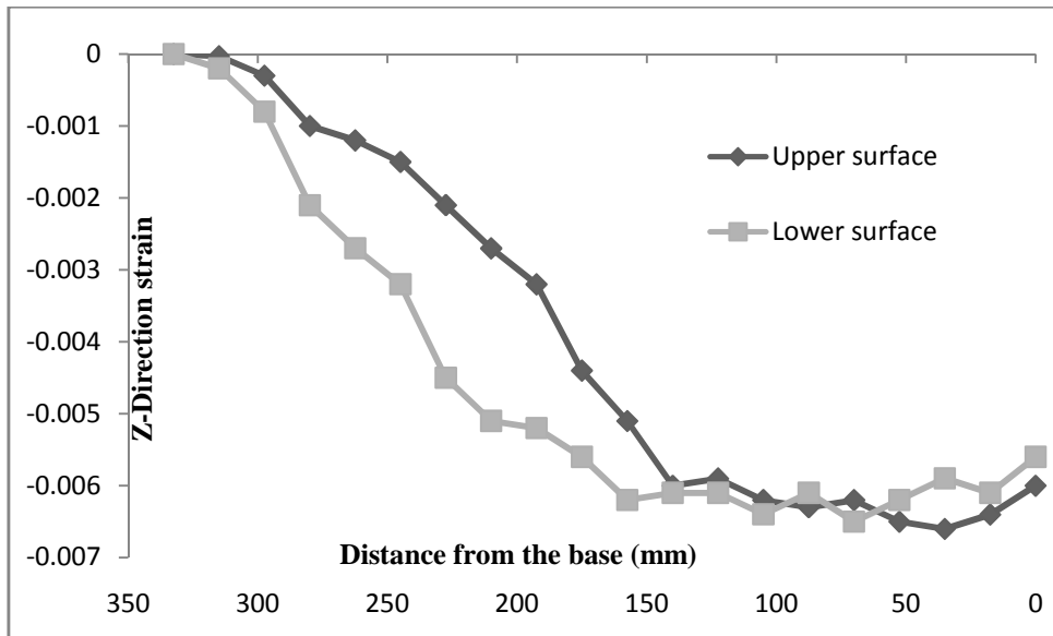
Figure 10. Z- Strain distribution on length
