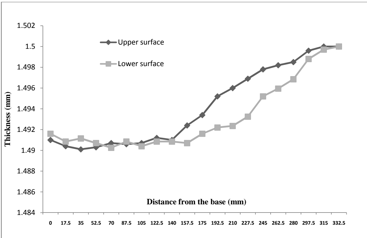
Figure 12. Thickness distribution on length
