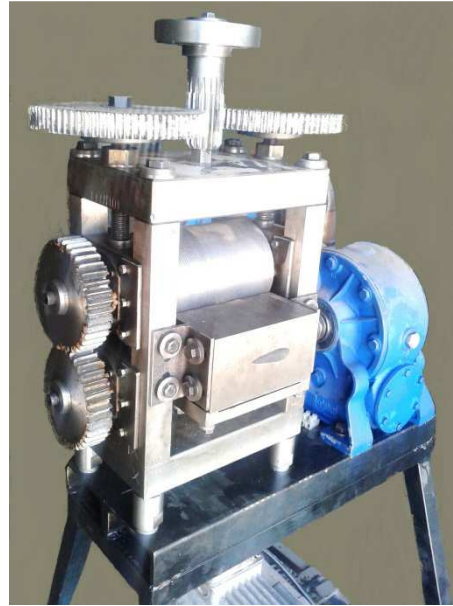
Fig.4. ECAR device
