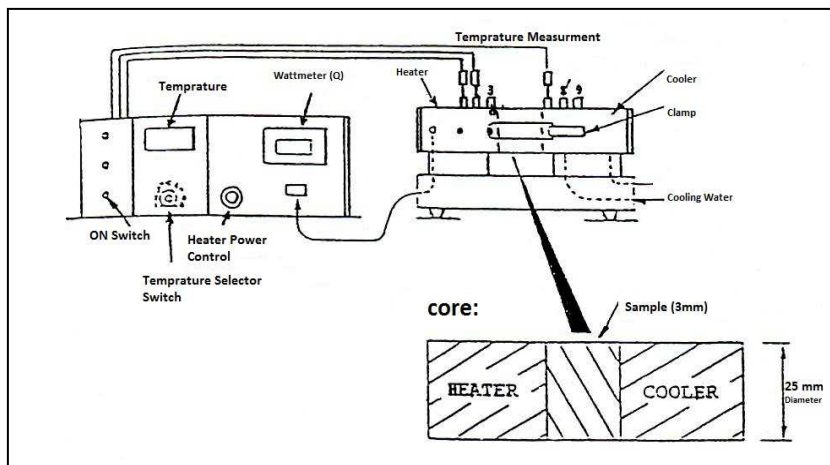
Fig.7. A schematic of Heat conduction apparatus
