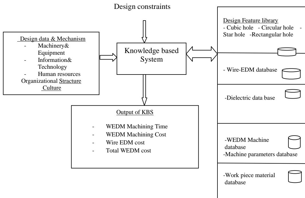
Figure4. Input, Output, constraint and databases of IKBS
