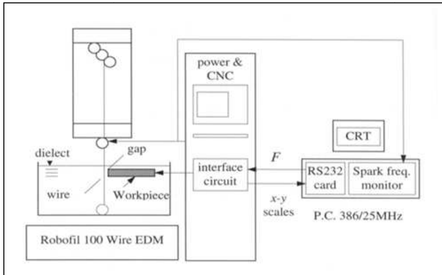
Figure2. Schematic diagram of process in WEDM
