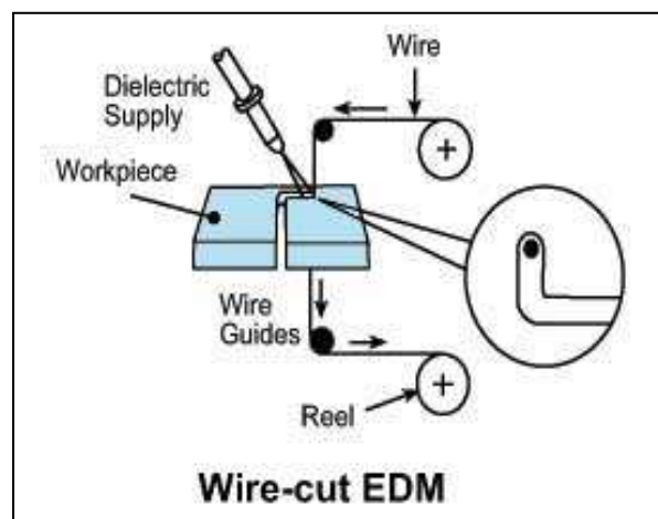
Figure 1. Schematic diagram of WEDM
